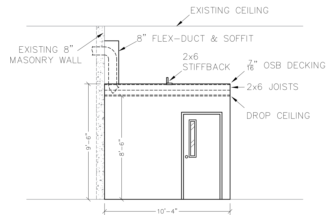
A5.3 NEW OFFICE ELEVATION 1 SCALE: 1/4" = 1'-0"
