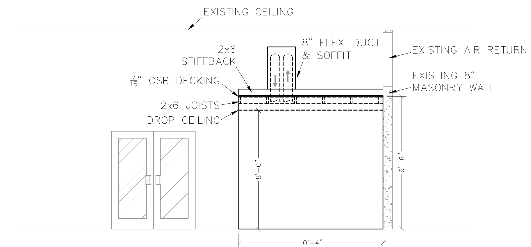
A5.4 NEW OFFICE ELEVATION 2 SCALE: 1/4" = 1'-0"
