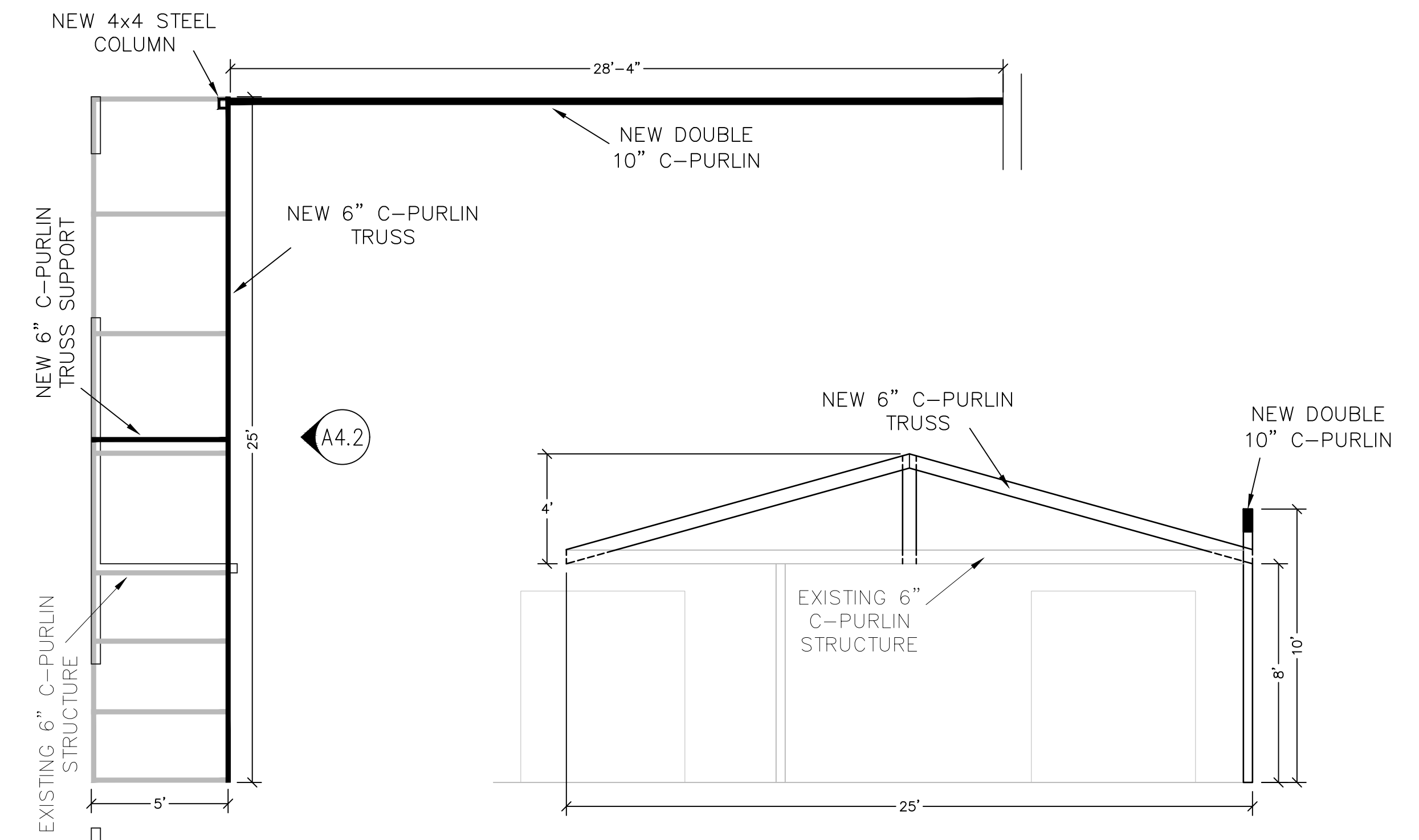
A4.2 MEZZANINE 2 - EXISTING AND NEW STEEL SCALE: 1/4" = 1'-0"
