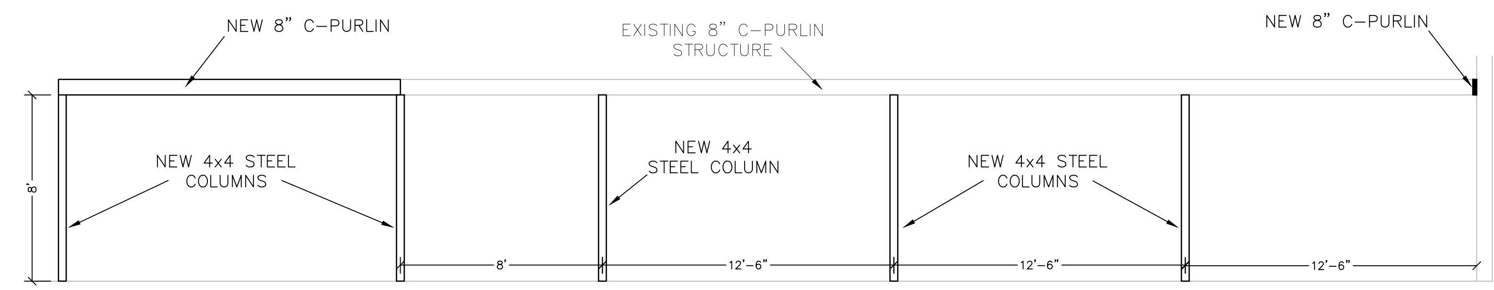
A4.1 MEZZANINE 1 - EXISTING AND NEW STEEL SCALE: 1/4" = 1'-0"
