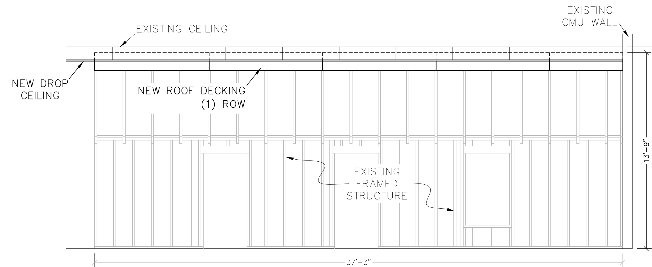
A5.2 FRAMED STRUCTURE INTEGRATION WITH DROP CEILING SCALE: 1/4" = 1'-0"
