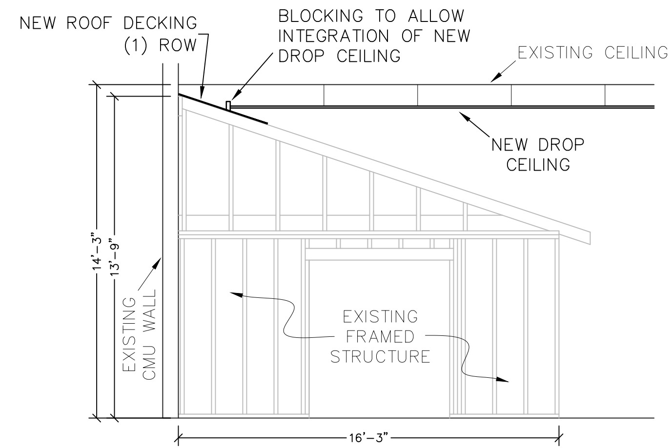
A5.1 FRAMED STRUCTURE INTEGRATION WITH DROP CEILING SCALE: 1/4" = 1'-0"
