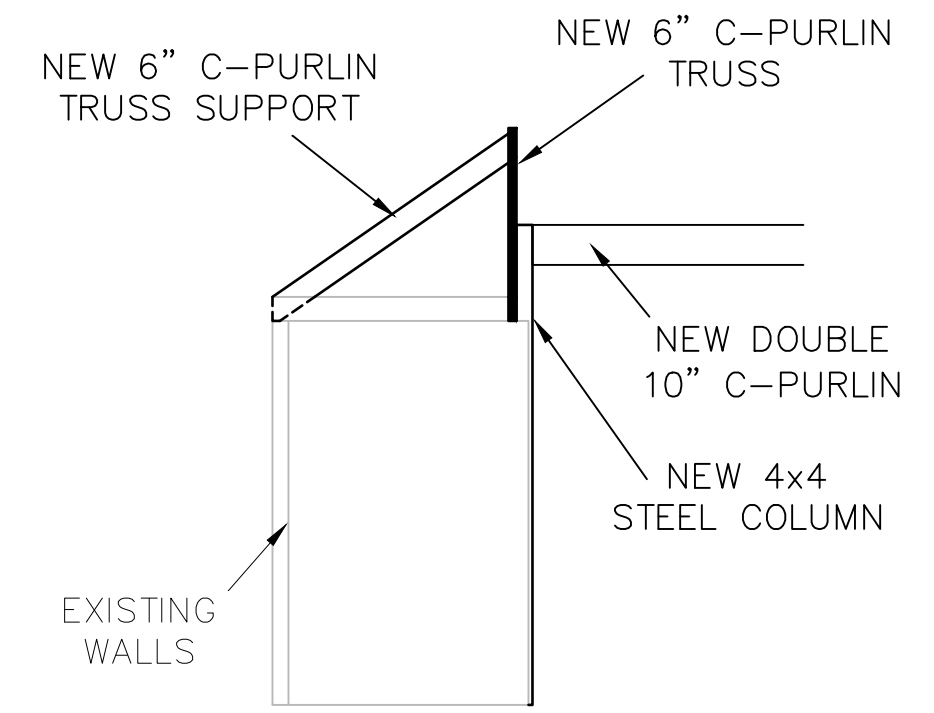
A4.3 MEZZANINE 2 - TRUSS SUPPORT SCALE: 1/4" = 1'-0"
